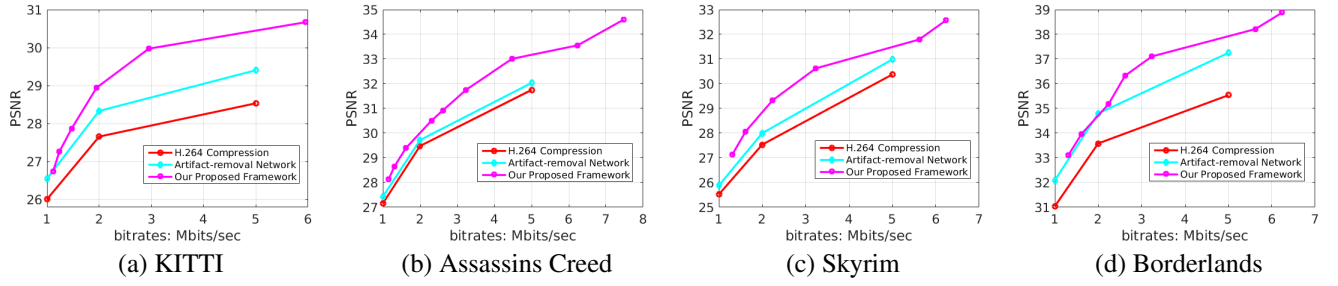
Figure 3: PSNR comparisons on four datasets at different bandwidths. We compare our pipeline with H.264 and an artifact-removal method based on (?; ?).
